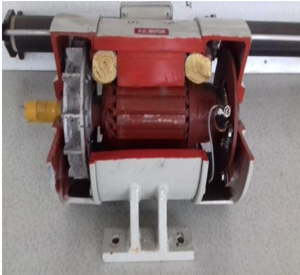
Cut- Set Model of DC Motor
