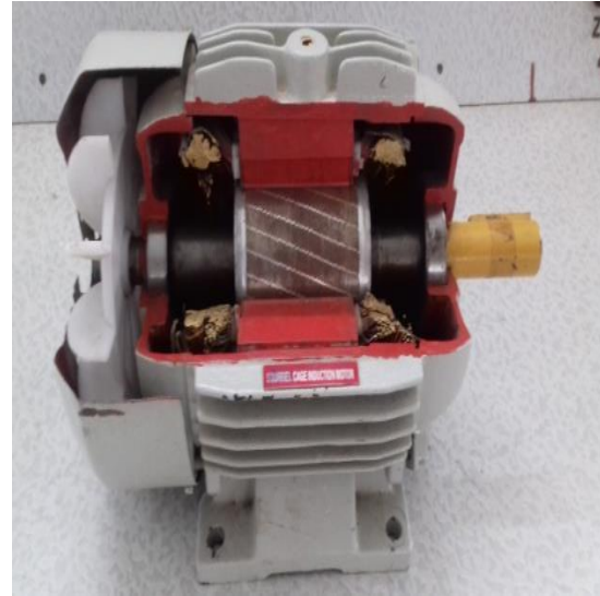
Cut- Set Model of Squirrel Cage Induction Motor
